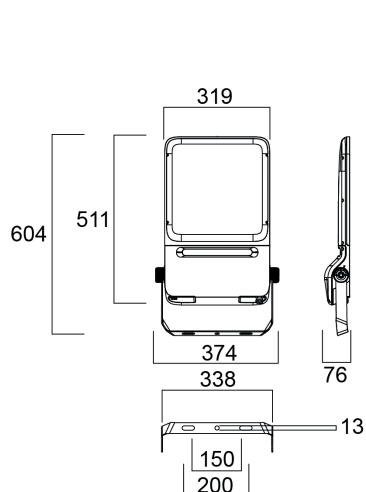
Concord Raiden 12000 / 21000 lm
