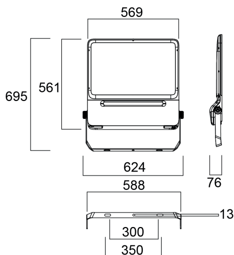
Concord Raiden 30000 / 40000 / 50000 lm
