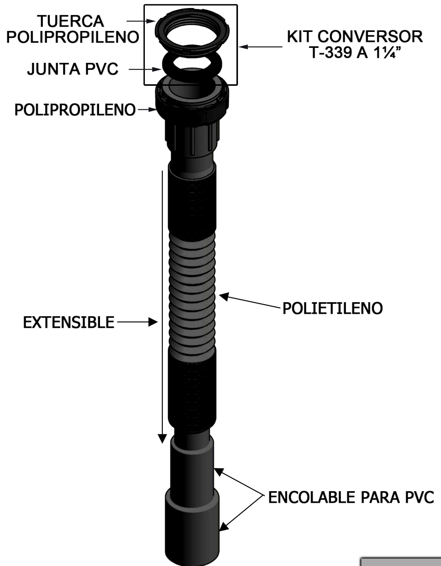
DESPIECE
